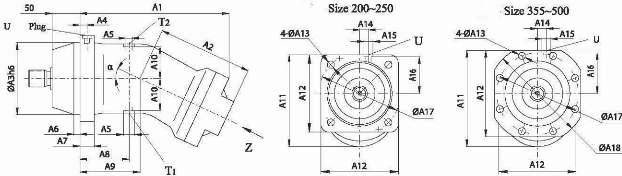
End Plate(Direction Z)
