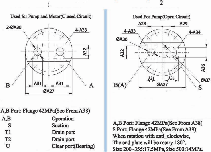
Series 5 Size 200~500 Table Of Unit Dimensions
