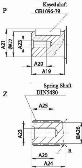
shaft end
